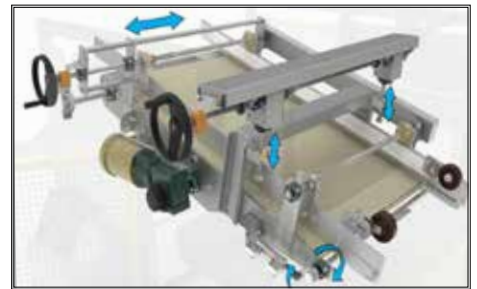
Lid Motion and Positioning Height Adjustment Mechanism
