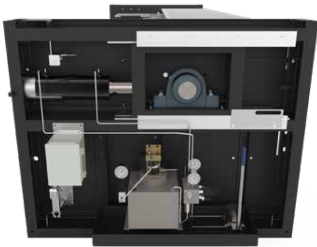
Newly Upgraded Hydraulic Tensioning Kit
