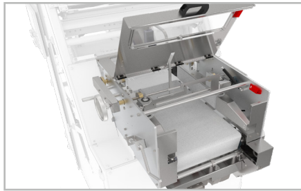
Belt Infeed Conveyor
