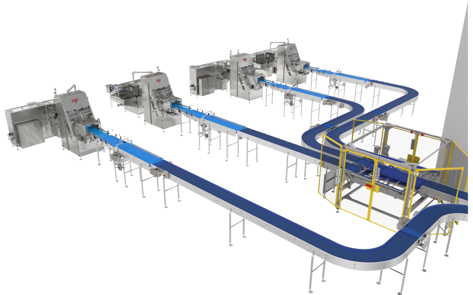
System Integration : Combo Slicer-Bagger with Slicer Feed Conveyor
