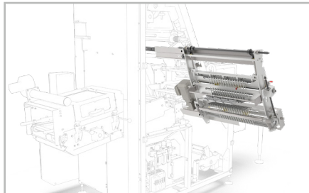
Heavy Duty Self Supporting Heavy Duty Lattice Pull-out Mechanism
