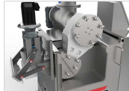
Vane Style Metering Pump
