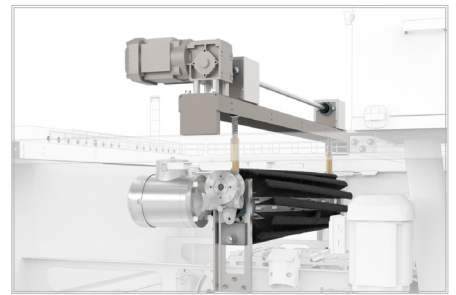
Automatic Brush Height Adjustment
