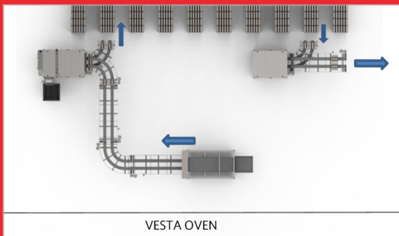
UPSIDE DOWN PAN STORAGE
