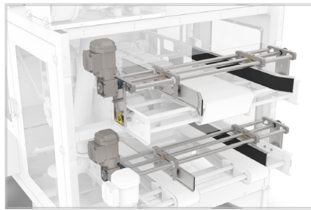
Automatic In and Out Guides Adjustment
